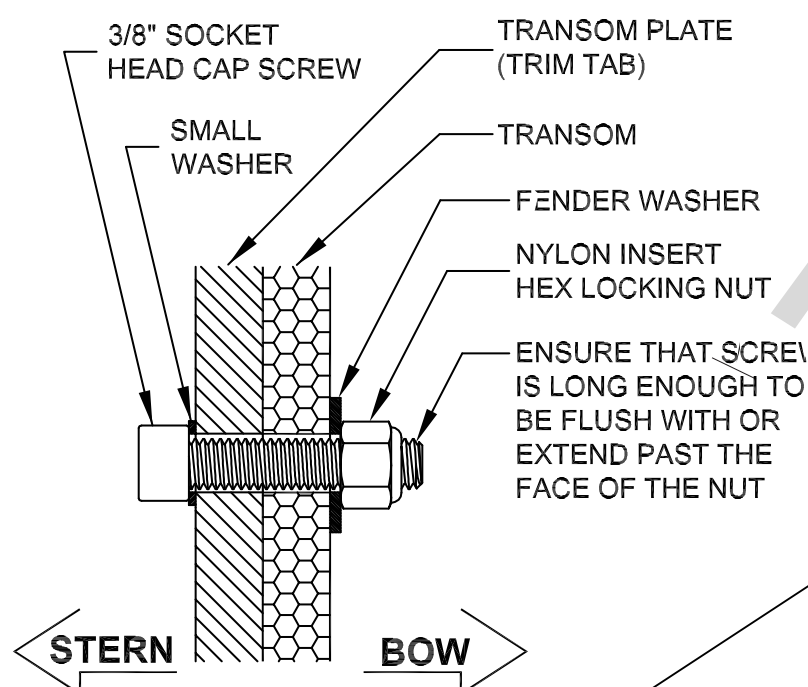
TYPICAL FASTENER INSTALLATION
