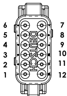
WIRE INSERTION VIEW
