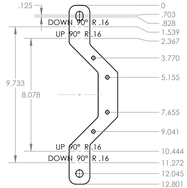
FLAT PATTERN VIEW FOR REFERENCE
