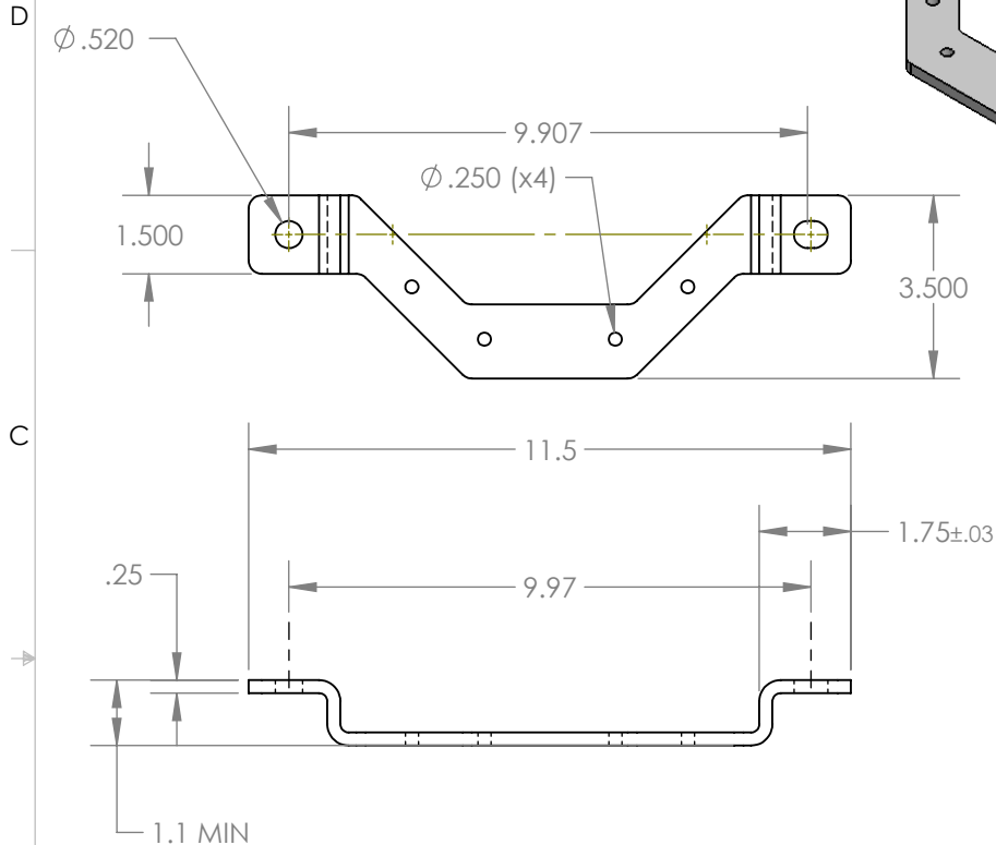
FORMED VIEW
